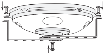
Horizontal Mount (two brackets)
